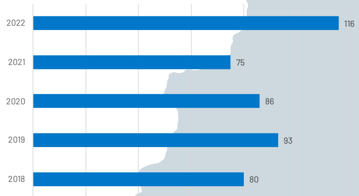
Represented Languages
